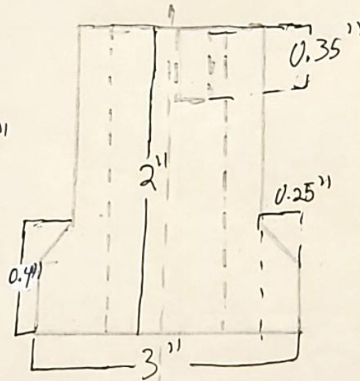
Slider Cup Right View
