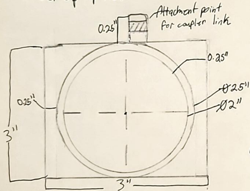
Slider Cup Top View
